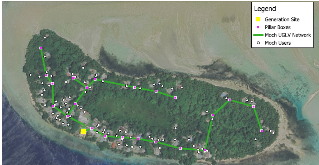
Figure 13. Mini-grid overview of Moch
