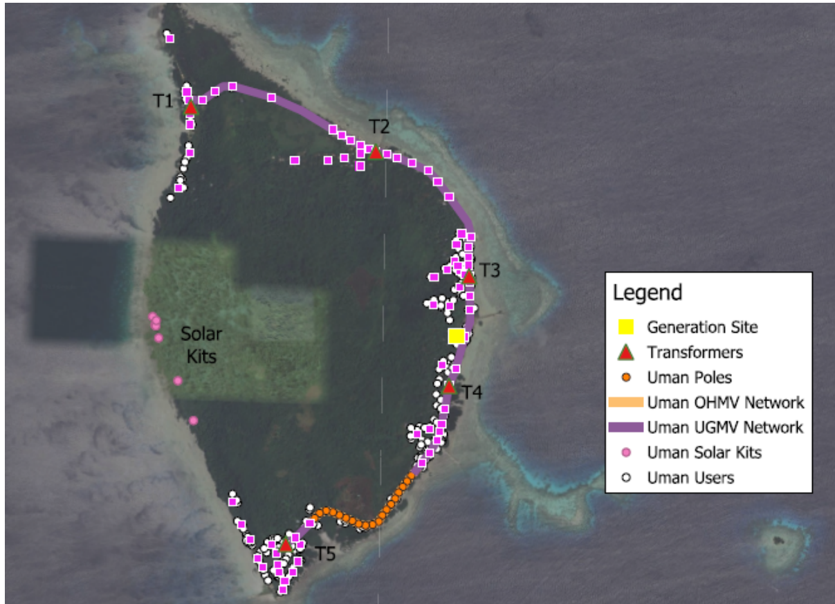
Figure 4. Mini-grid overview of Uman
