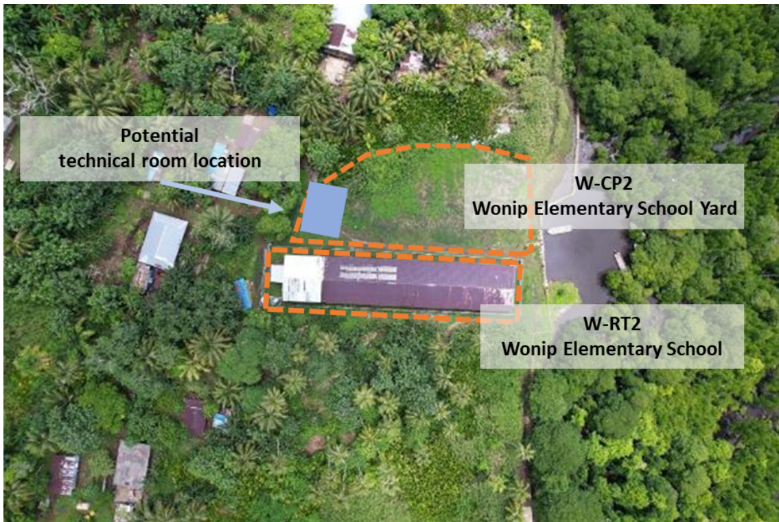
Figure 8. Aerial view of the proposed generation PV site 2 (G2) for Tol (Wonip)
